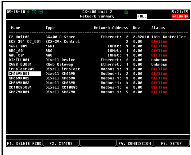
Figure 18-6 - Network Summary Screen
