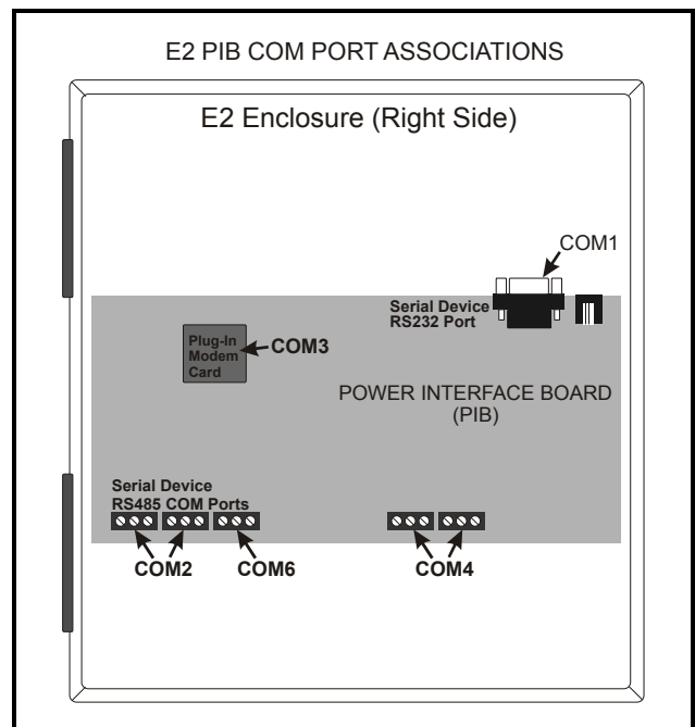
Figure 18-3 - Location of E2 COM Ports - E2 PIB (E2 versions 4.2 and above)
