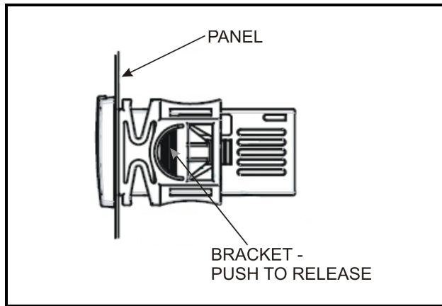
Figure 11-1 - Installation and Mounting of XR35CX
