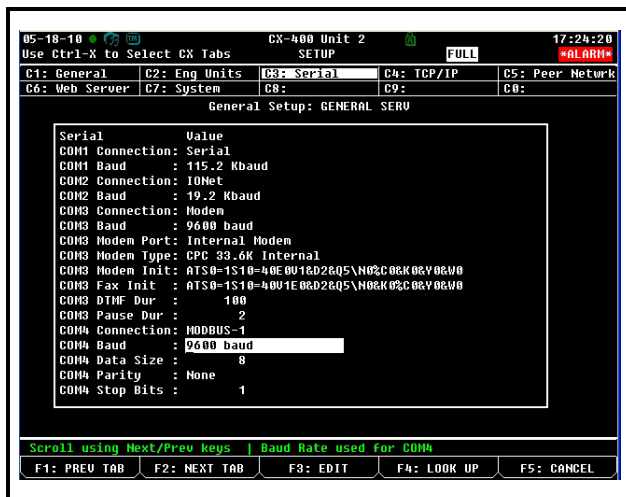
Figure 18-4 - Serial Communications Manager Screen
