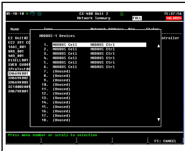
Figure 18-7 - List of MODBUS Devices
