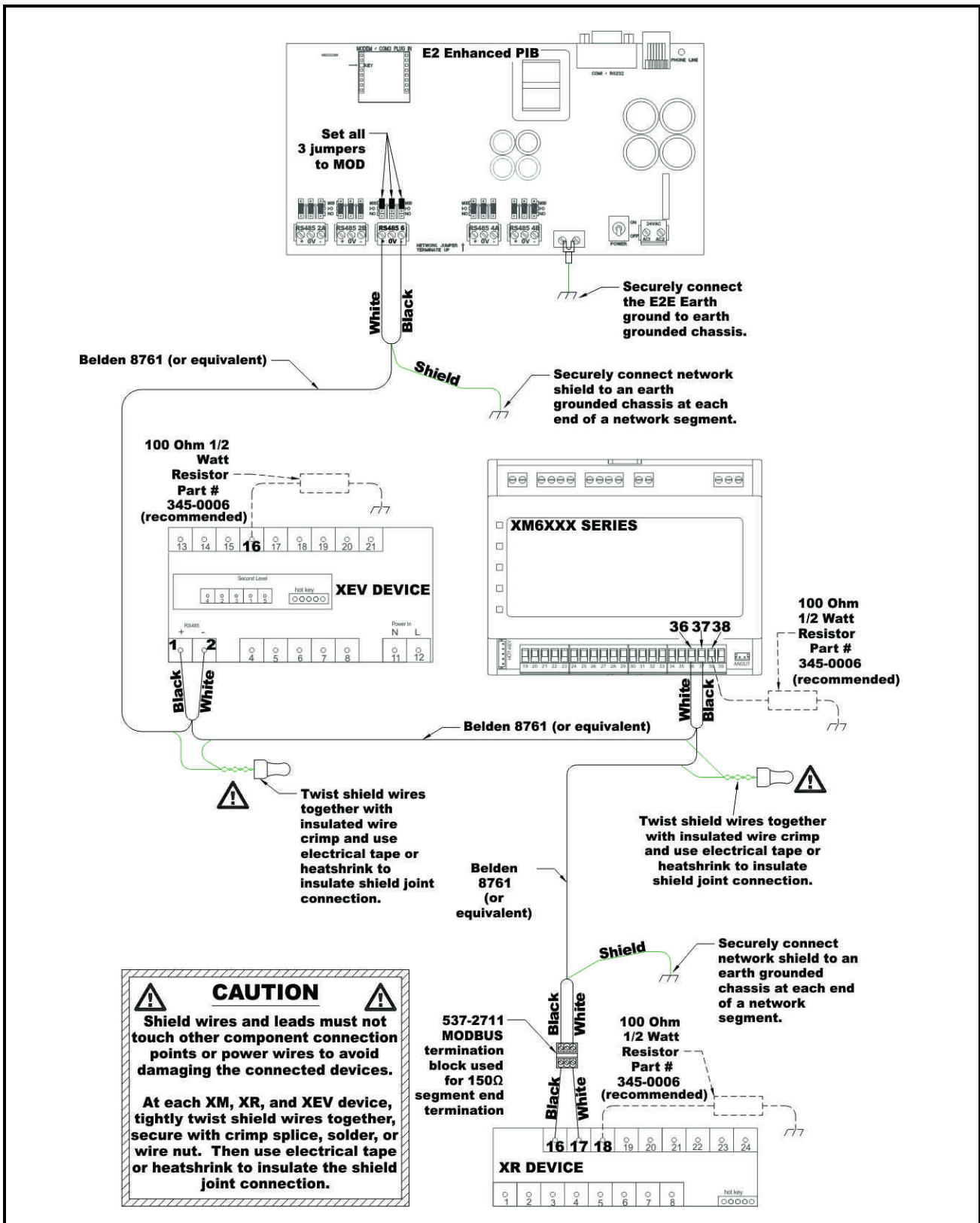
Figure A -I - MODBUS Com Wiring Diagram
