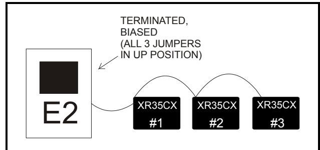
Figure 18-2 - MODBUS Networking
