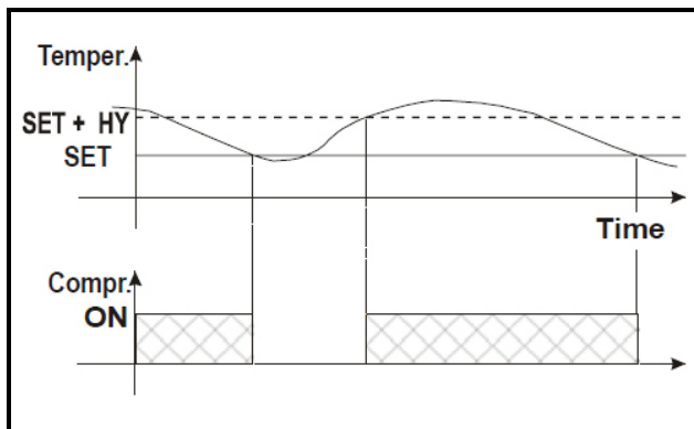
Figure 3-1 - Compressor Temperature Regulation
