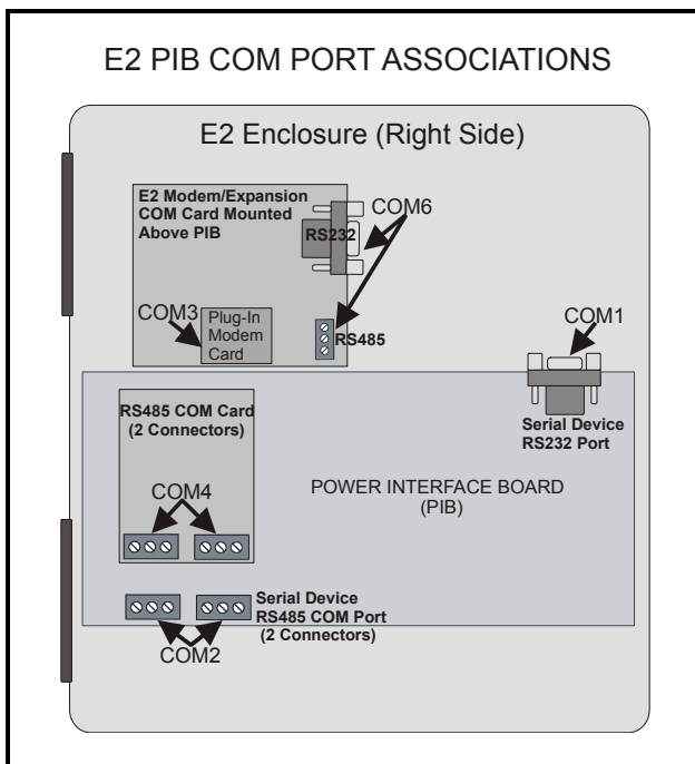
Figure 18-1 - Location of E2 COM Ports (E2 versions 3.xx and below)
