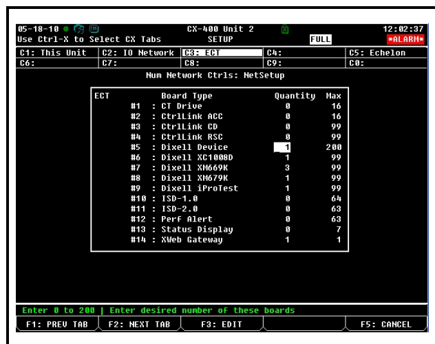
Figure 18-5 - Num Network Ctrls: NetSetup Screen
