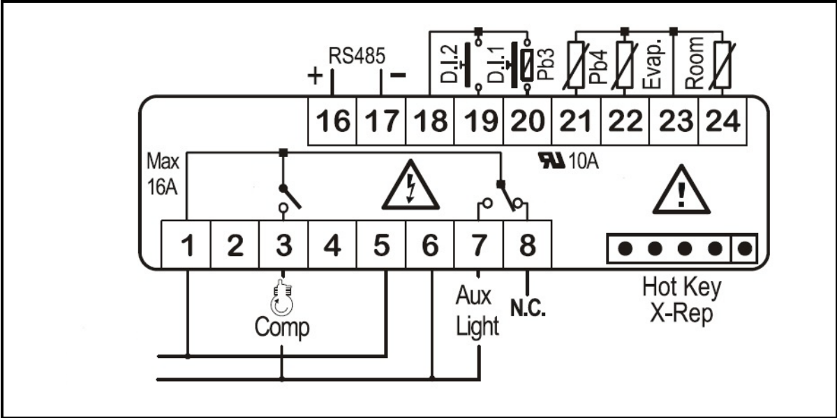
Figure 16-1 - XR35CX Connections
