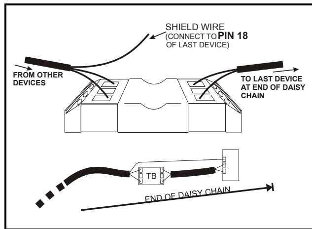
Figure 18-9 - MODBUS Termination Block ( P/N 535-2711 )
