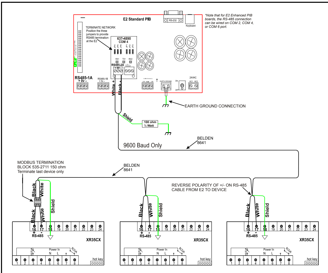
Figure 17-1 - XR35CX to E2 MODBUS Network Wiring
